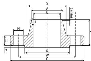
WN Welding Neck
