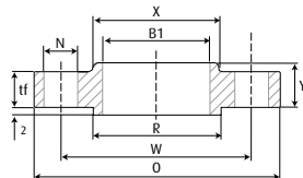
SO Slip on
