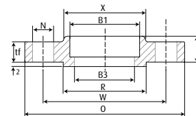
SW Socket Welding
